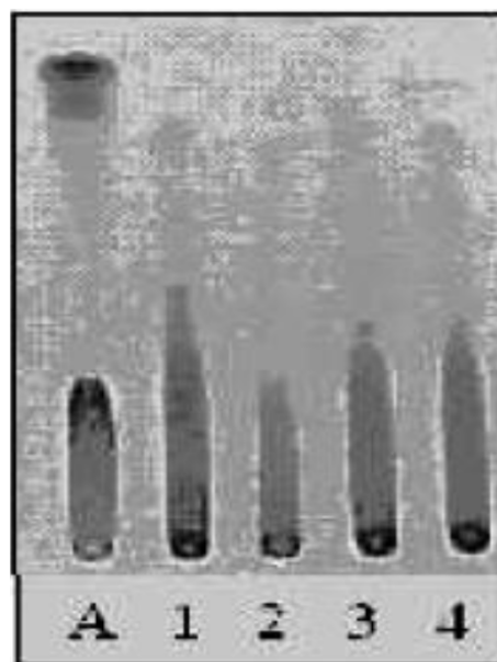
Figure 1: TLC ethanol extract from cashew husk (1-dry and milled: 2-dry and entire: 3-natural and milled: 4-natural and entire: A-tannic acid standard).
