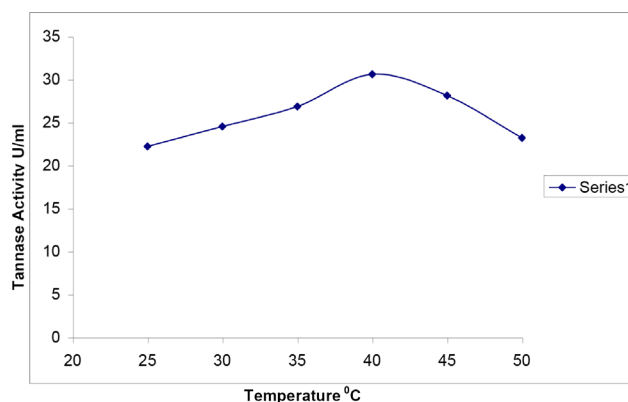
Figure 3: Effect of Temperature on Tannase production.
