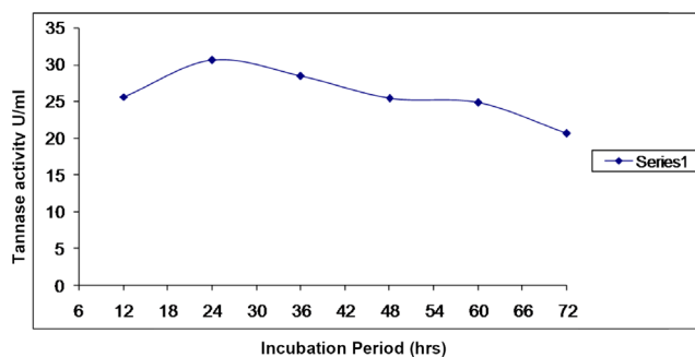
Figure 1: Effect of Incubation period on Tannase production.
